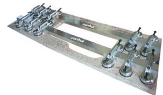
WEHA Suction Cup Assembly
